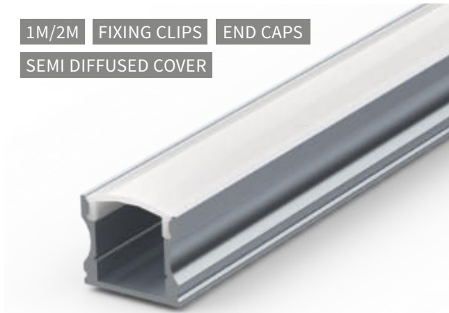
Deep Surface | W: 17.3mm x H: 14.5mm Code: P-DS-1 / P-DS-2
