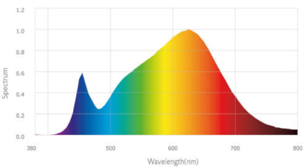
■ SPECTRAL RADIANT FLUX VERSUS WAVELENGTH
