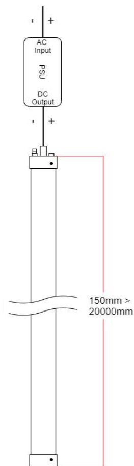
■ WIRING DIAGRAM
