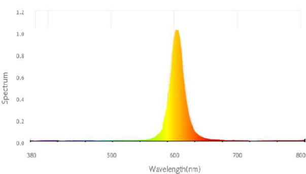
■ SPECTRAL RADIANT FLUX VERSUS WAVELENGTH
